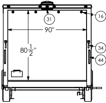
EXTERIOR REAR
