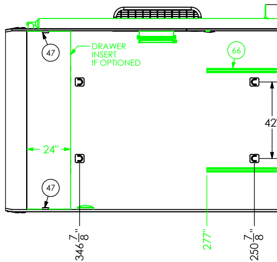
STRAIGHT BASE CABINET AGAINST RISER WALL OR DELETED BASE CABINET OPTION
