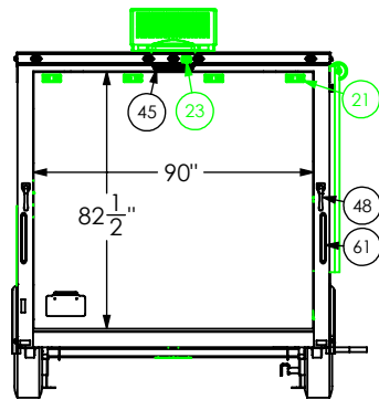
EXTERIOR REAR
