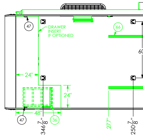
L-BASE FRONT CABINET W/ GEN BOX AND DOOR
